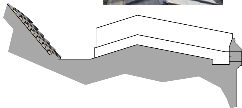
SECTION THROUGH ORGAN CHAMBER ROOF SHOWING EAST PARAPET
